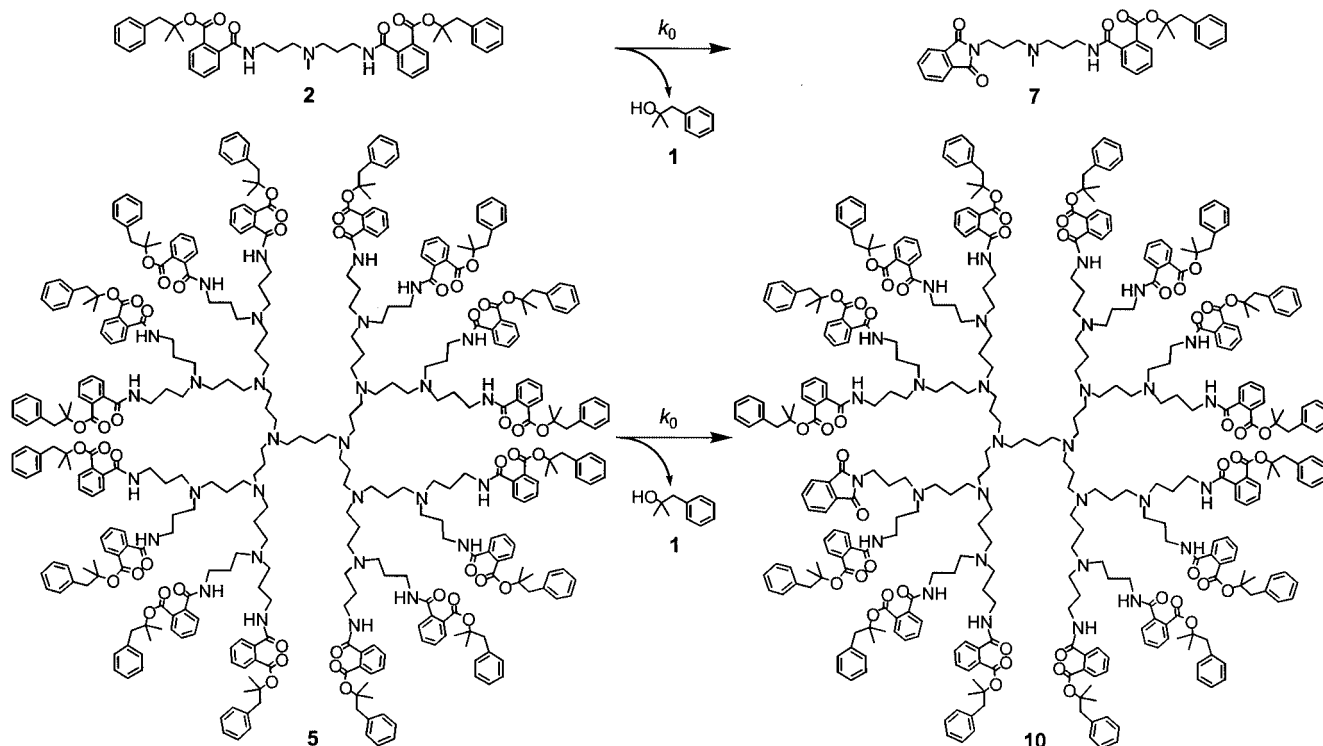
Scheme 3. Schematic representation of the first step in the neighbouring group assisted release of alcohol 1 from precursors 2 and 5
