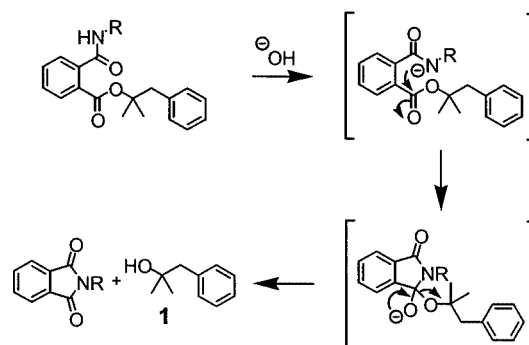
Scheme 1. Neighbouring group assisted cyclisation of 2-carbamoylbenzoates for the release of tertiary fragrance alcohol 1
