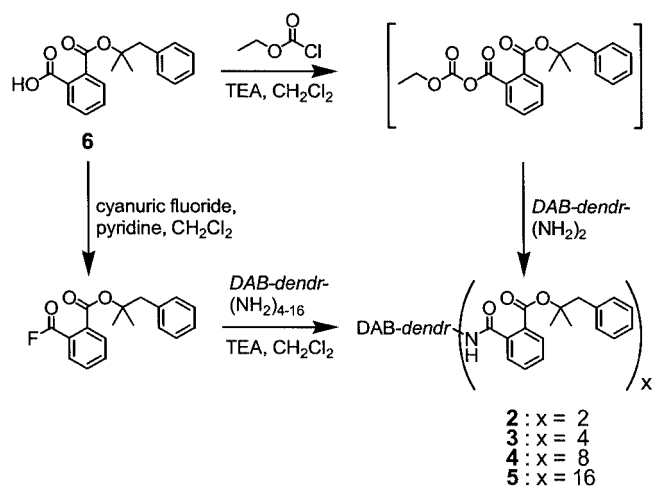
Scheme 2. Preparation of dendritic 2-carbamoylbenzoates 2–5 from (1,1-dimethyl-2-phenylethyl) hydrogen phthalate ( 6 )
