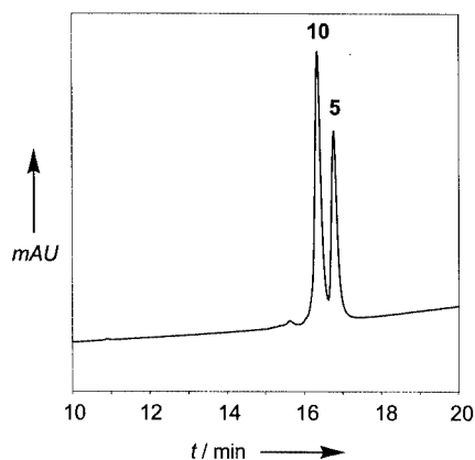
Figure 1. Analytical HPLC trace (conditions see Exp. Sect.) obtained for the co-injection of two pure preparative MPLC fractions, containing monocyclused dendrimer 10 and its noncyclised precursor 5 , respectively
